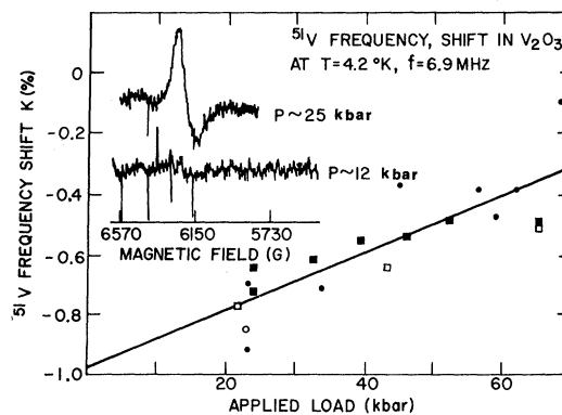
FIG. 2. ^{51}\text{V} frequency shifts in \text{V}_2\text{O}_3 at T = 4.2^\circ\text{K} and f = 6.9 MHz. Circles and squares refer to measurements taken, respectively, on the initial application of load and on a second application of load two days later. Closed data points refer to measurements made with increasing load and open data points to measurements with decreasing load. A later measurement on a third sample using spin-echo amplitude measurements at 26 kbar gave K(26 \text{ kbar}) = -0.92\% \pm 0.20\% . The calibration of the load was obtained from the 25.5-kbar transition of bismuth on the initial loading, as described in the text. During the second loading (square data points) it was noted that the bismuth transition was reached under \sim 20\% less load than on the initial loading. For this reason, the pressure on the \text{V}_2\text{O}_3 sample in the 20- to 30-kbar regime is as much as 5 kbar greater than indicated for the square points. Conversely, in the regime above 50 kbar, cracking of the girdle may have resulted in a reduction of pressure. Correction for these two effects would raise the already anomalously high slope shown for the frequency shift versus pressure. It is also probable that in the presence of pressure inhomogeneities in the 20- to 30-kbar regime the portions of the sample in the higher-pressure regions would contribute more strongly to the observed resonance than would those portions of sample in lower-pressure regions. This phenomenon would result from the rapid falloff in resonance intensity at low pressures demonstrated in Fig. 3 and in the inset of this figure. For this reason, also, the data points in the 20- to 30-kbar regime may represent pressures up to 5 kbar greater than shown. Consideration of such a correction would also increase the frequency-shift-versus-pressure slope. The inset of the figure shows free-induction-decay nuclear-resonance amplitudes as measured with phase-coherent detection at 25 and 12 kbar. The greatly reduced amplitude at 12 kbar results from the fact that the sample is antiferromagnetically ordered at this pressure, and the nuclear resonance is consequently shifted out of the region of observability to a much higher frequency.
