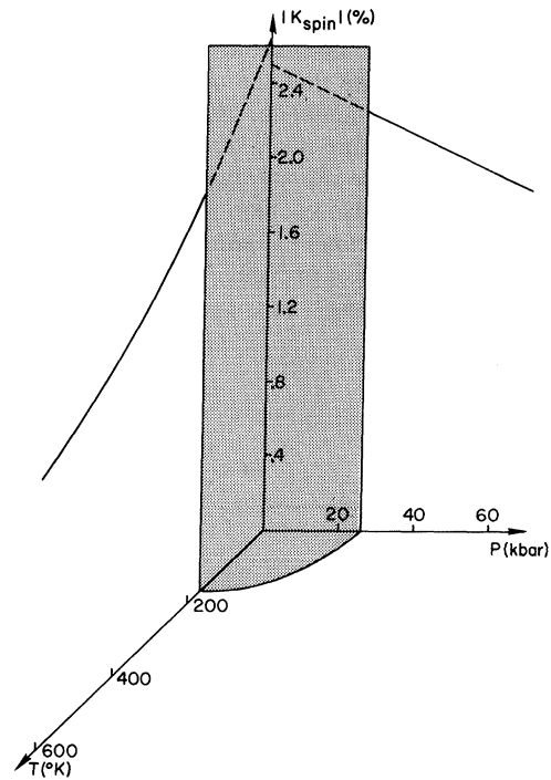
FIG. 4. d -spin components of ^{51}\text{V} NMR frequency shifts as a function of pressure at T = 4.2 °K and as a function of temperature at P = 1 atm. The solid lines are linear and Curie-Weiss fits, respectively, of the data. The broken lines are continuations of the fits in the anti-ferromagnetic region where no resonances were observed.
